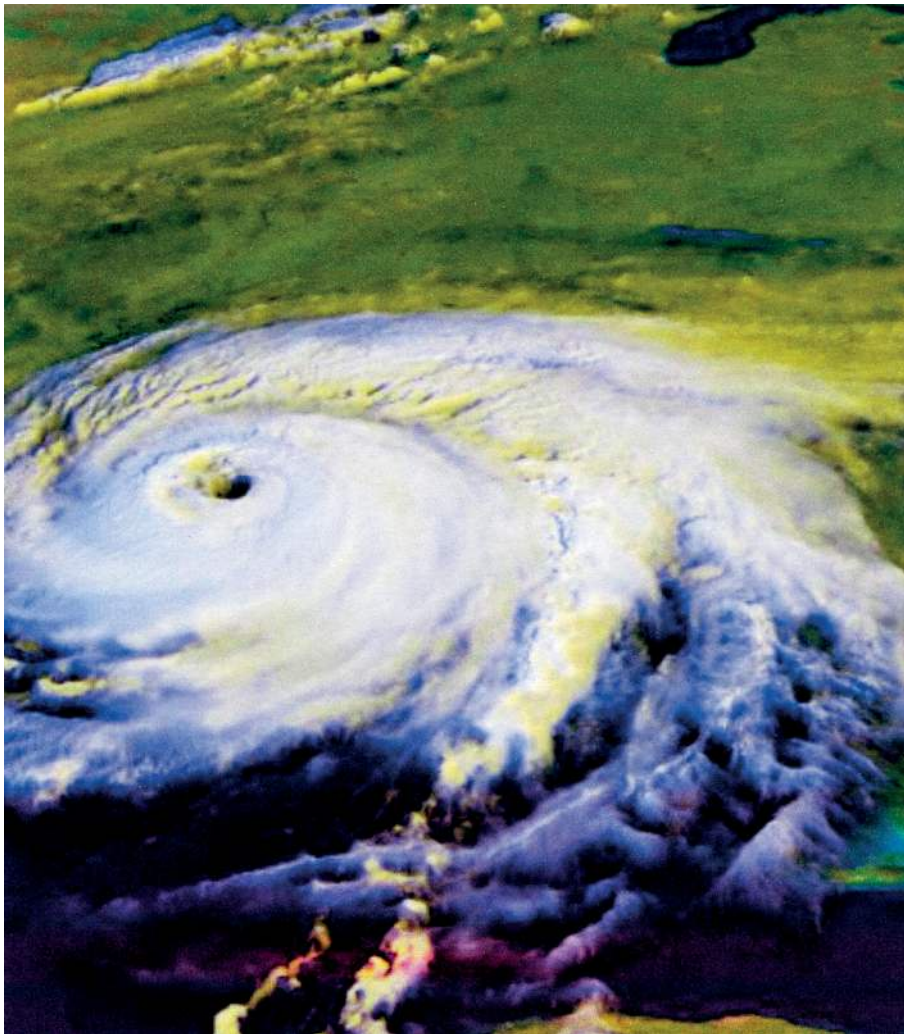
Satellite image of a tropical storm, 'hurricane Ivan'
